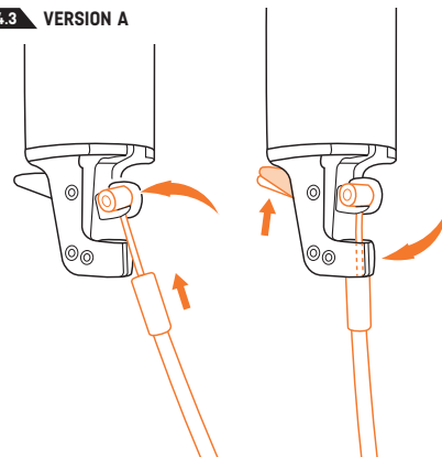
4.3 VERSION A
