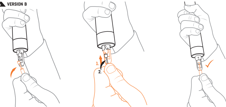
3.4 VERSION B
