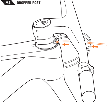
9.1 DROPPER POST
